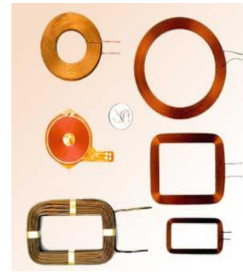
RF Coil Ass'y
