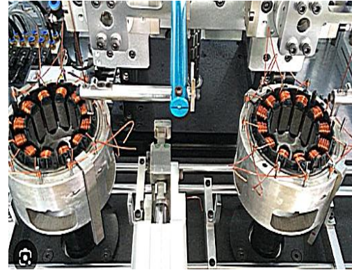
BLDC motor coil winding machine
